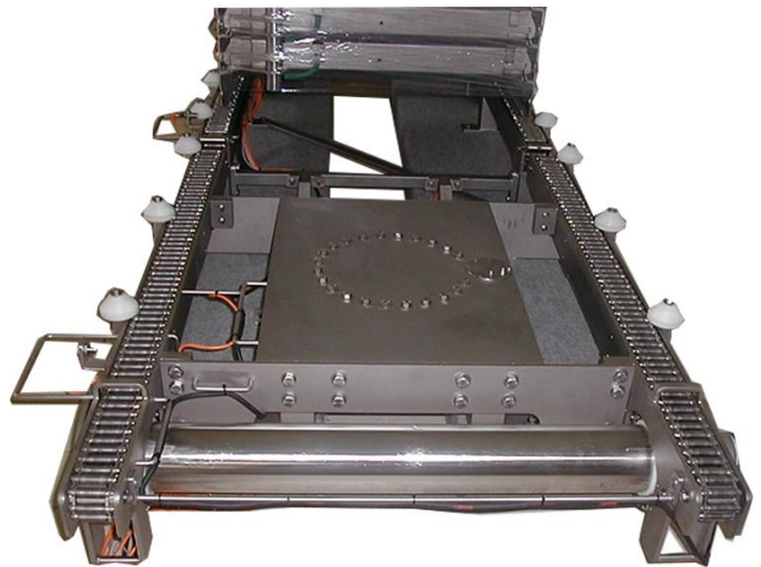
ROTATING UNIT Type RRSC For tranfer to 90° / 180° position Length according to customer's requirement Driven by an electrical motor
